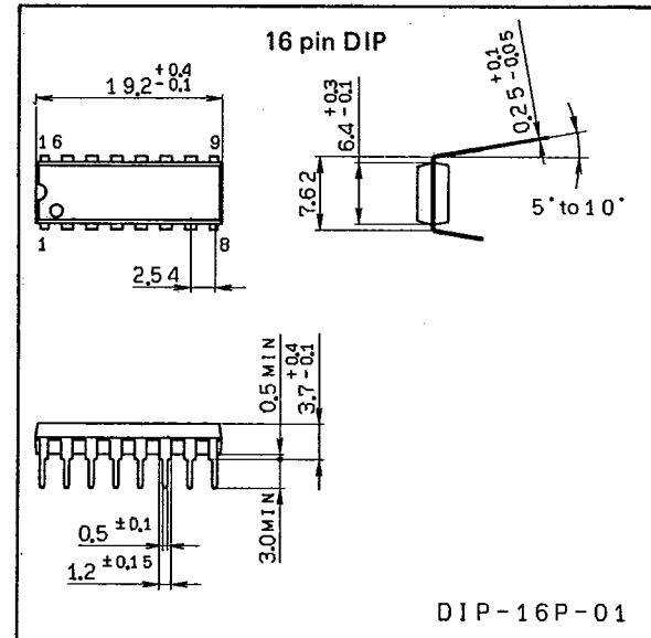
Package Outline
