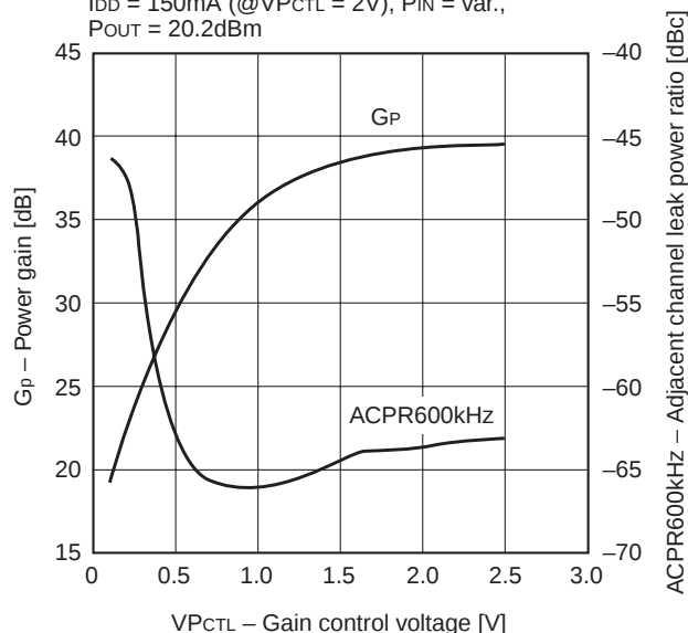
G_p , ACPR600kHz vs. V_{\text{PCTL}}
