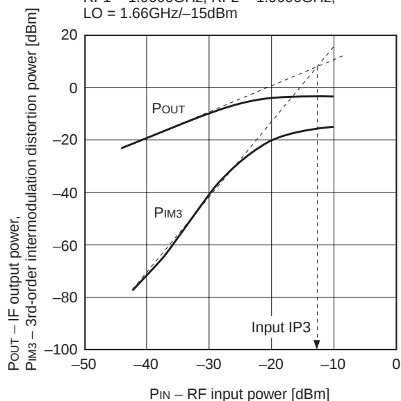
P OUT , P IM3 vs. P IN
