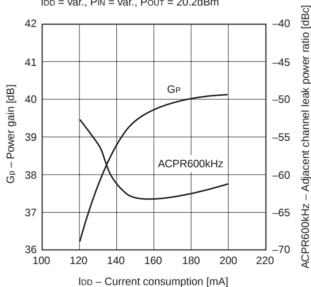
G_p , ACPR600kHz vs. I_{\text{DD}}
