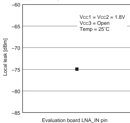
Graph 7. Local Leak
