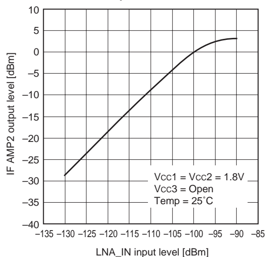
Graph 2. Total Gain
