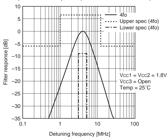
Graph 6. Filter Response (Normalized at 4.092MHz)
