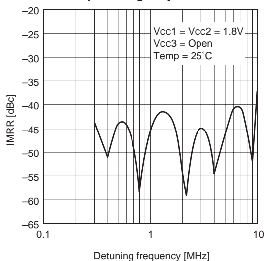
Graph 4. Image Rejection Ratio
