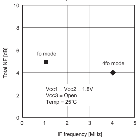
Graph 3. Total NF
