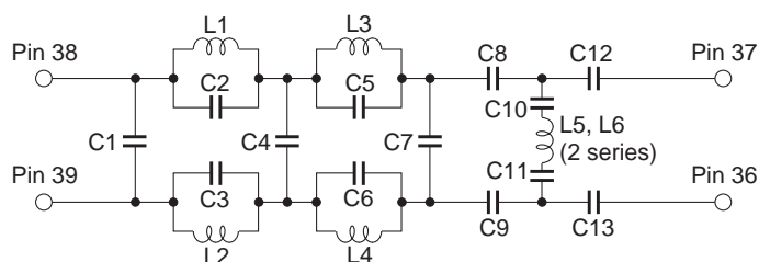
Overall External Filter Block
