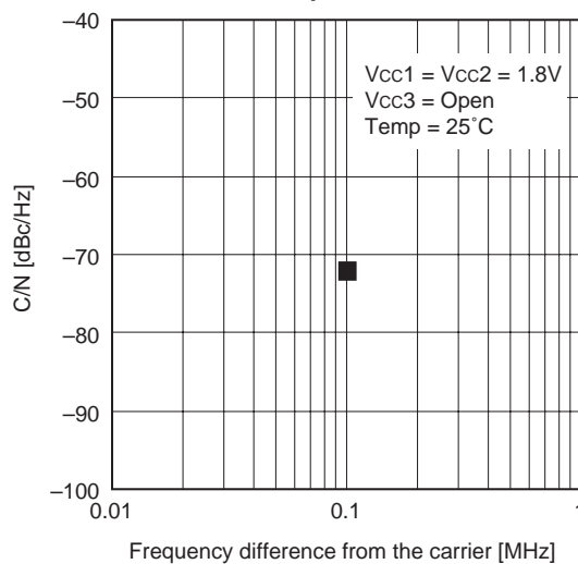
Graph 8. C/N
