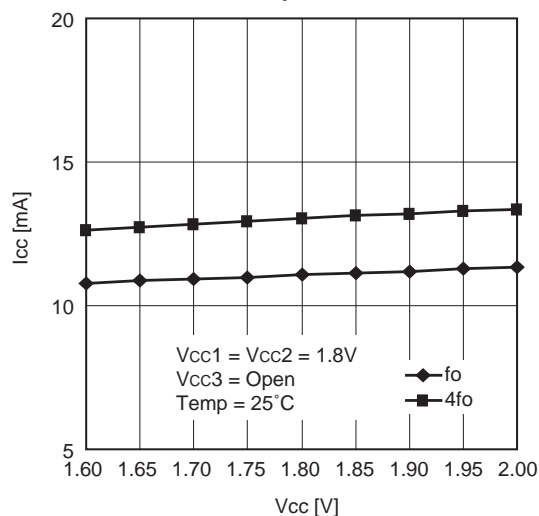
Graph 1. I cc
