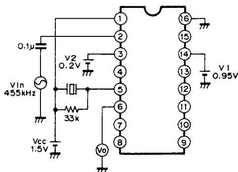
Test circuit 1
