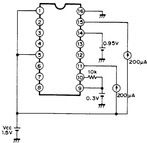
Test circuit 8
