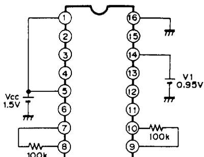
Test circuit 2
