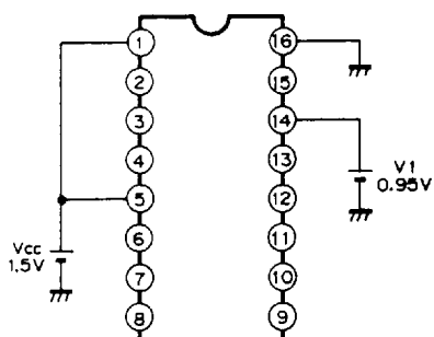
Test circuit 1
