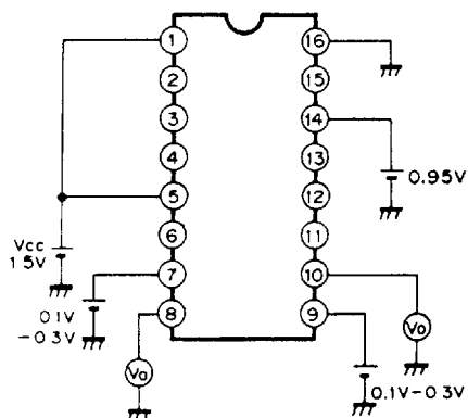
Test circuit 3
