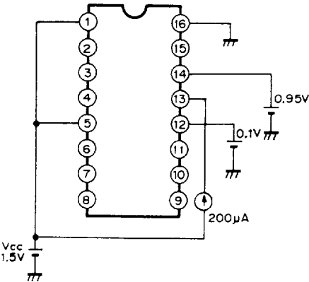
Test circuit 9
