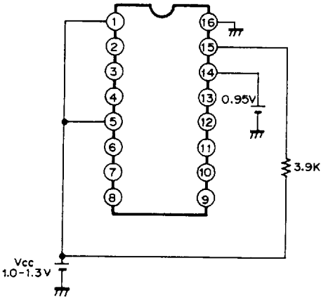
Test circuit 10
