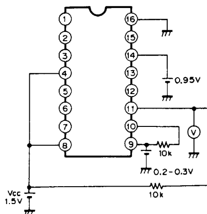
Test circuit 6
