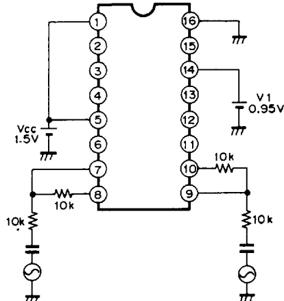
Test circuit 4
