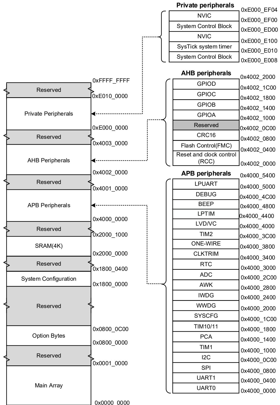
Fig. 3-2 Memory mapping
