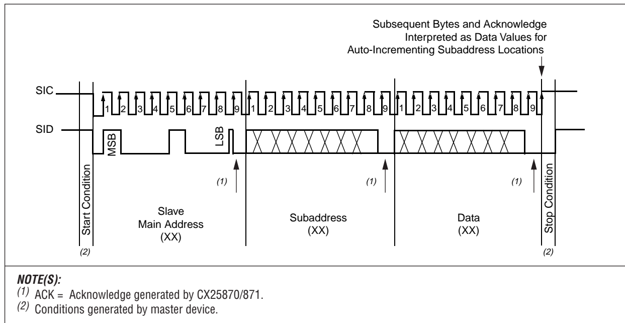
www.DataSheet4U.com Figure 3-16. SID/SIC Serial Programming Diagram
