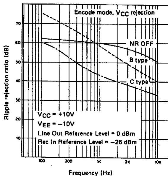
Ripple rejection ratio (1)
