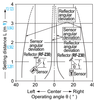
Retroreflective type
