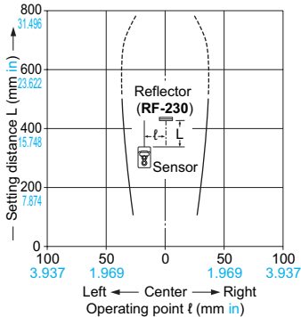
CX-424□
