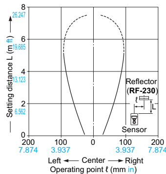
CX-482□
