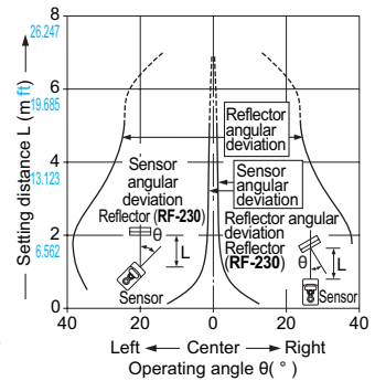
Retroreflective type
