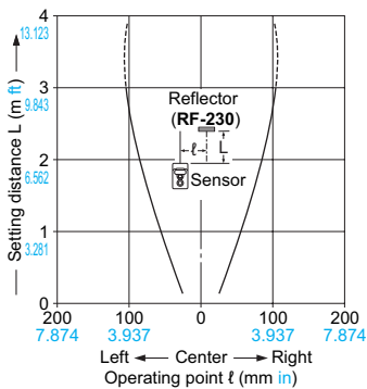
CX-481□
