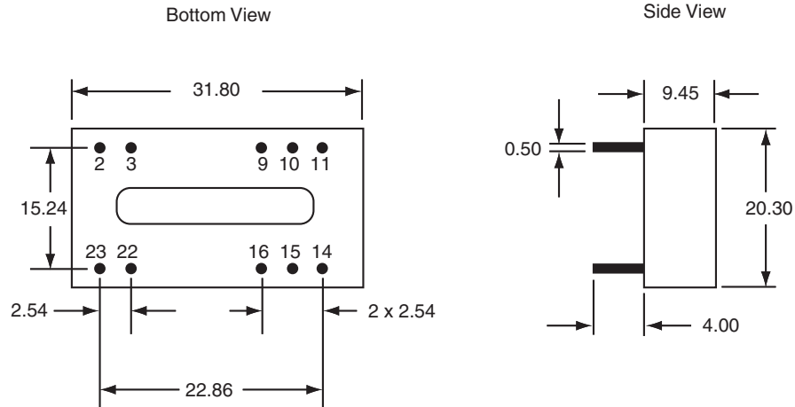
CTDD3120DF-S3K-3 Package
