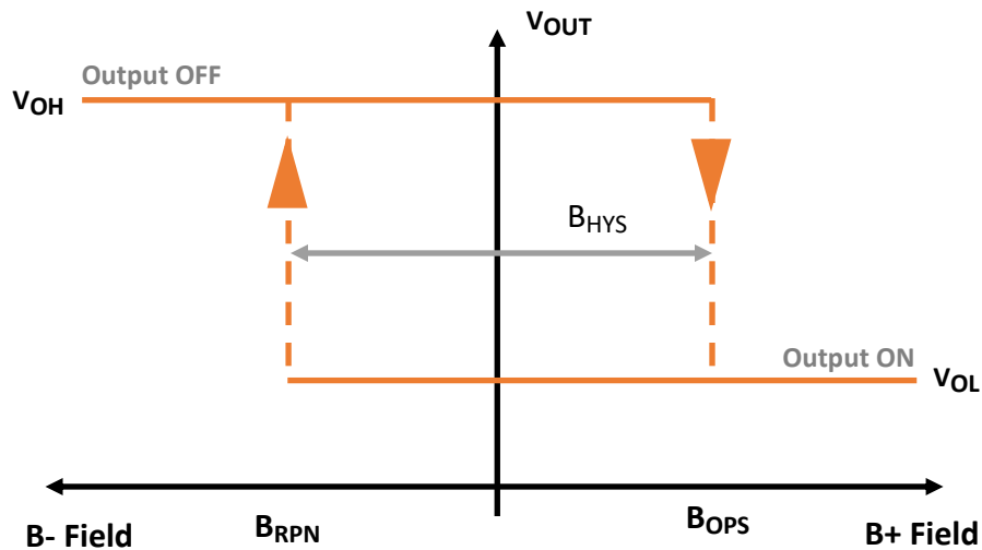
Output Behavior vs. Magnetic Field
