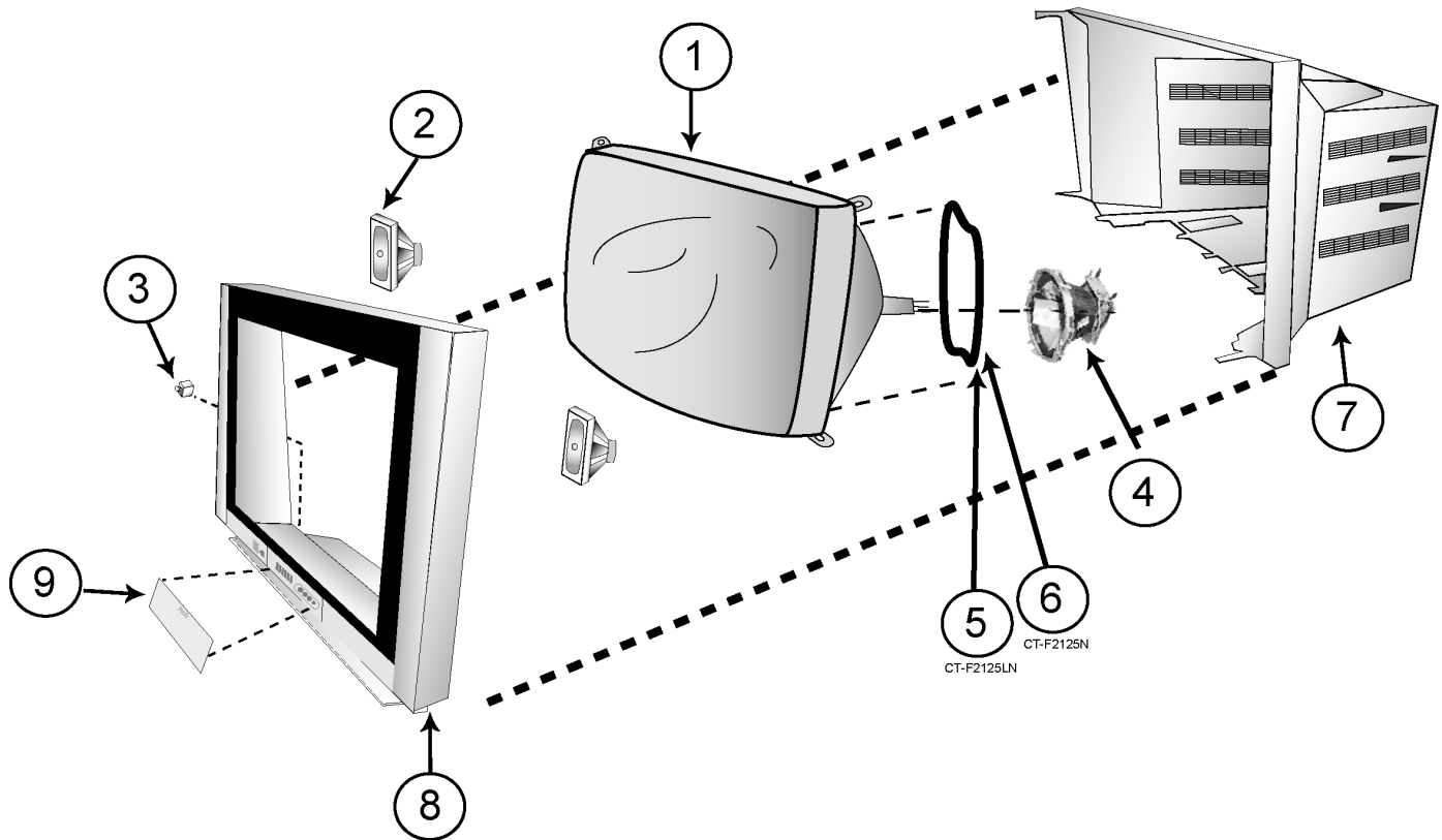
EXPLODED VIEW
