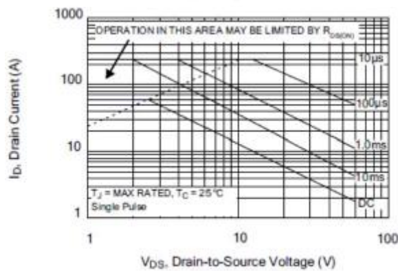
Figure 13. Maximum Forward Bias Safe Operating Area
