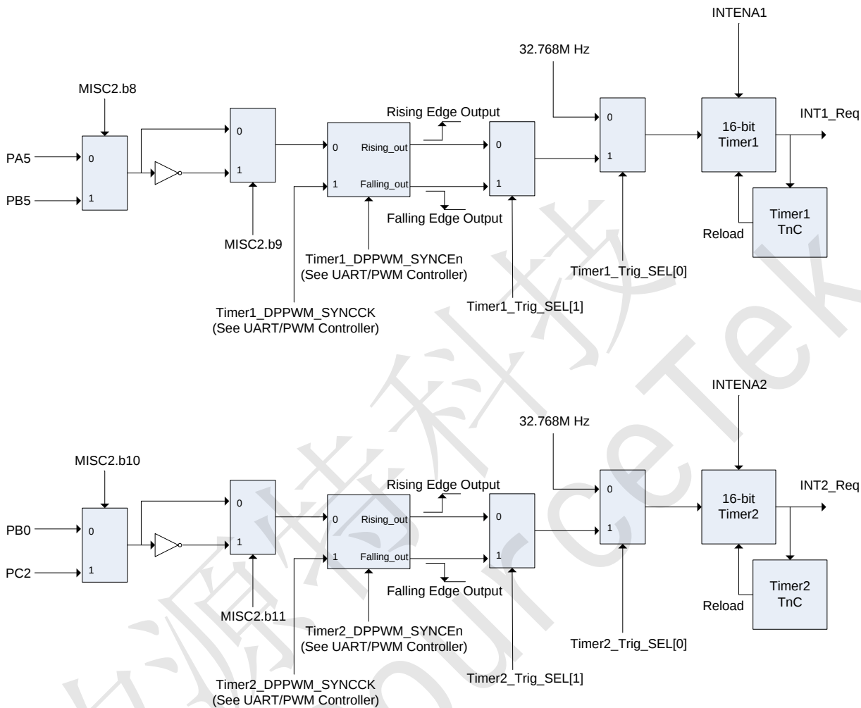
Figure 7.2 Timer1&Timer2 Structure
