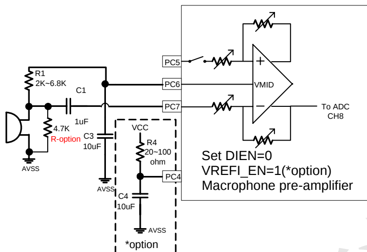
Fig 8.2 Microphone single end input application circuit
