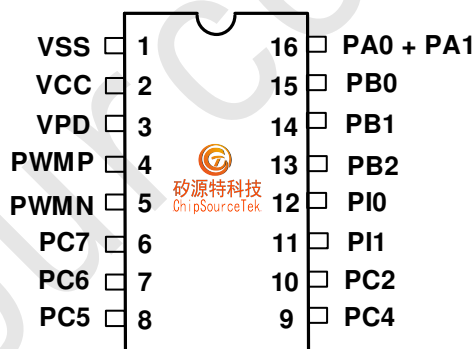
SOP16-3 (CST1604C)
