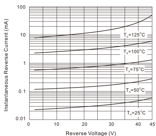
Fig. 3 - Reverse Characteristics
