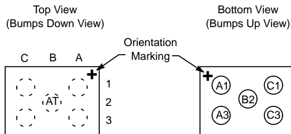
WLCSP5 Package
