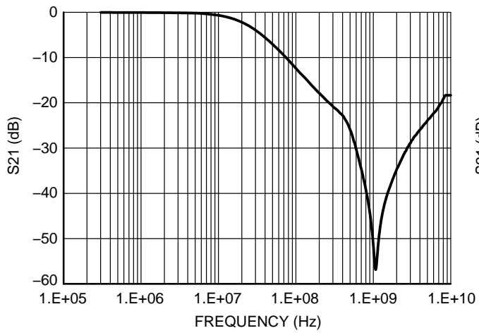
Figure 1. Typical Insertion Loss (50 \Omega Termination)
