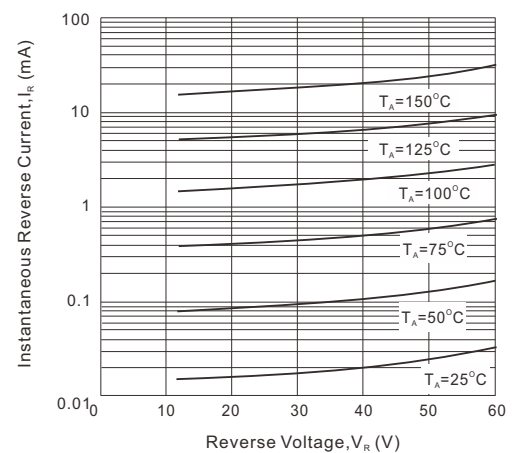
Fig. 3 - Reverse Characteristics
