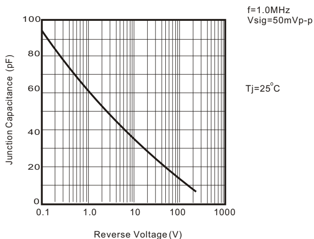
Fig. 3 - Junction Capacitance
