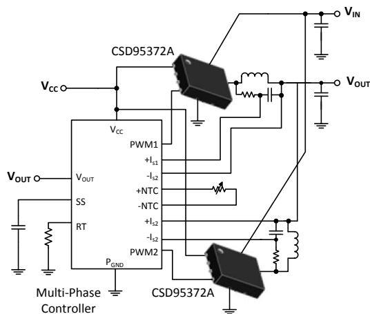
Application Diagram
