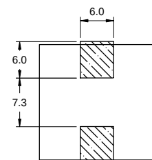
Typical Pad Layout
