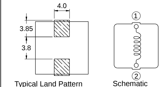
Typical Land Pattern
