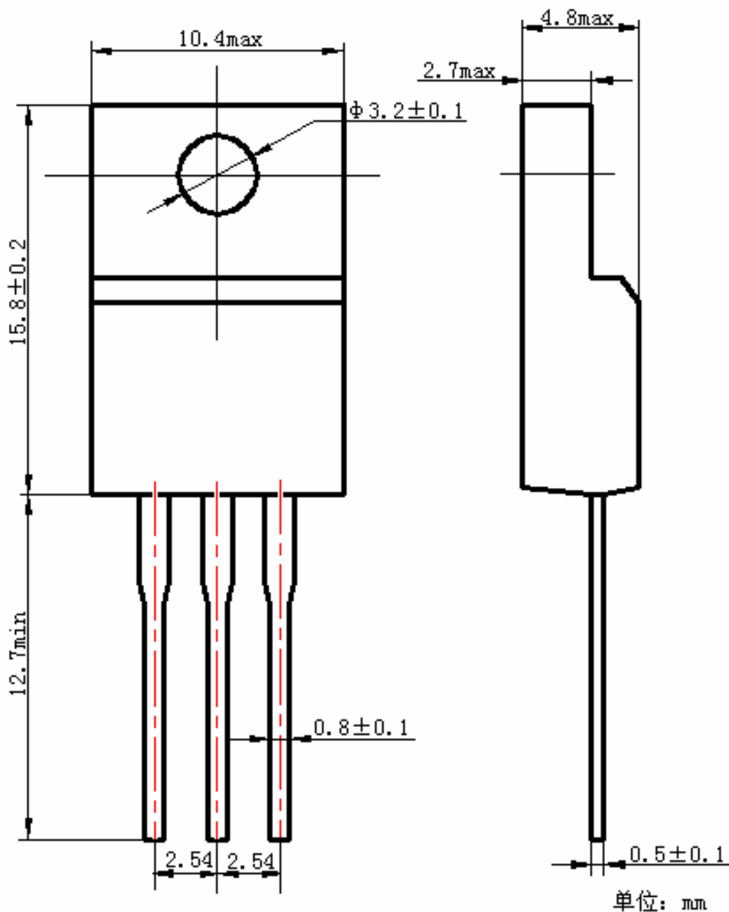
TO-220F Package
