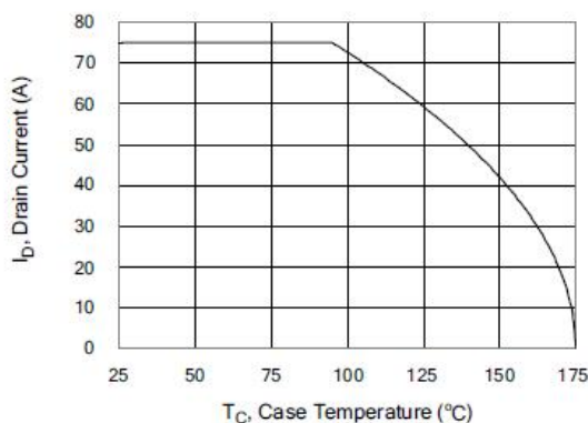
Figure 3. Maximum Continuous Drain Current vs Case Temperature
