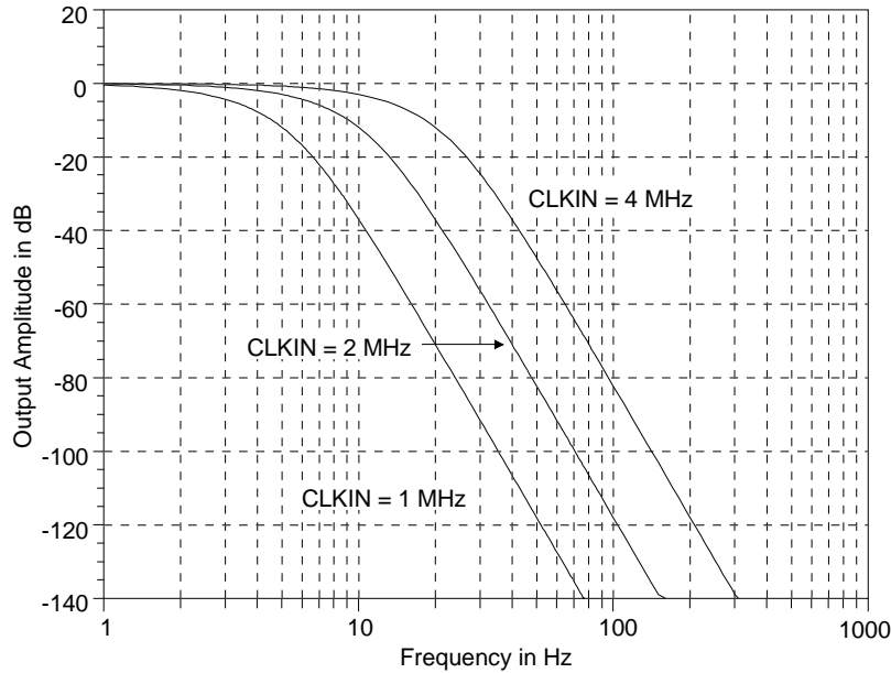
Frequency Response
