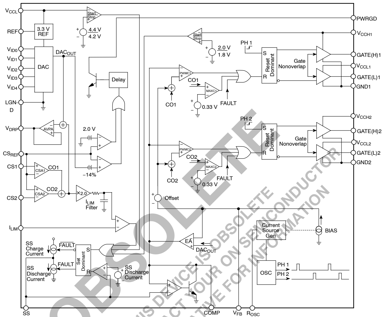
Figure 2. Block Diagram
