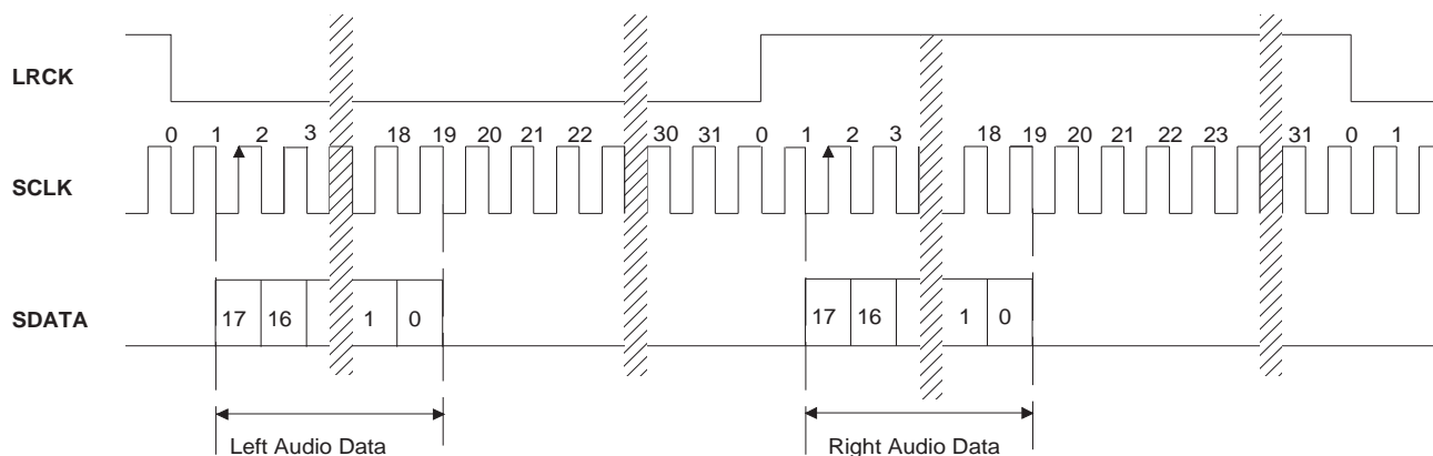
Figure 3. Data Output Timing - CS5331A (I²S Compatible)
