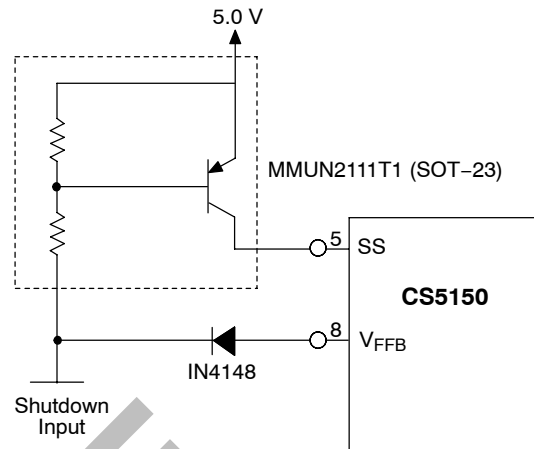
Figure 16. Implementing Shutdown with the CS5150
