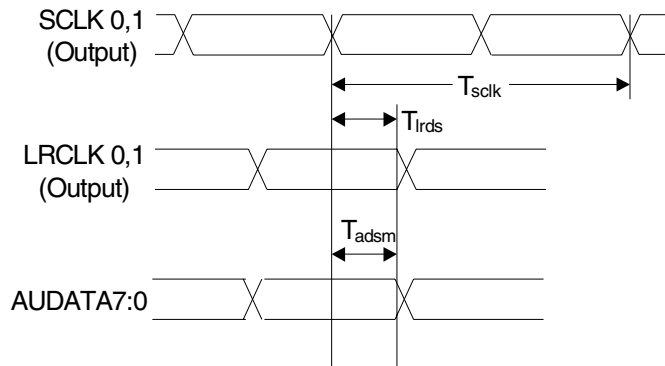
Master Mode (Output A1) Output Clock Timing and Digital Audio Output Data
