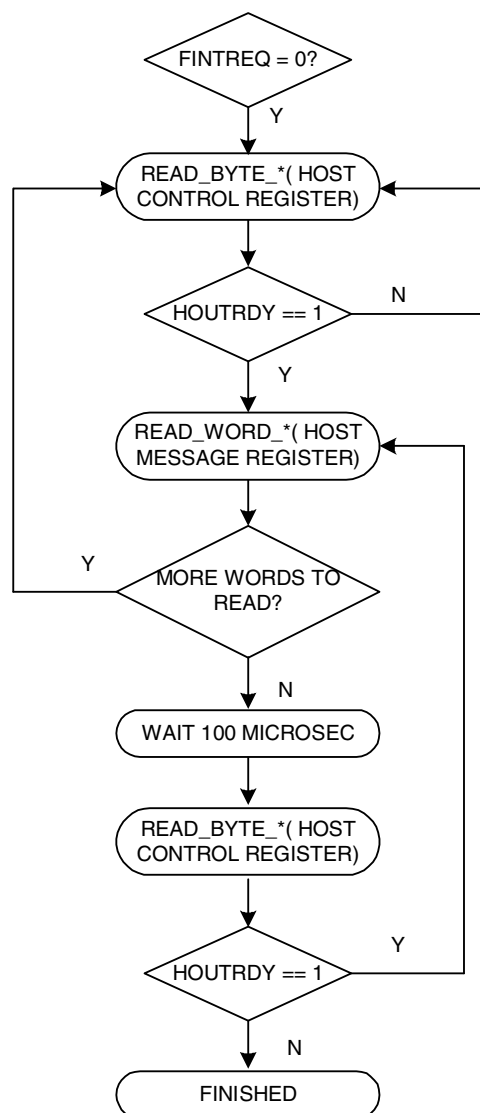
Figure 51. Typical Parallel Host Mode Control Read Sequence Flow Diagram for DSPC
