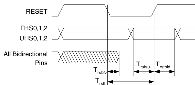
Figure 1. RESET Timing
