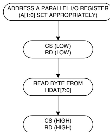
Figure 44. Intel Mode, One-Byte Read Flow Diagram for DSPC
