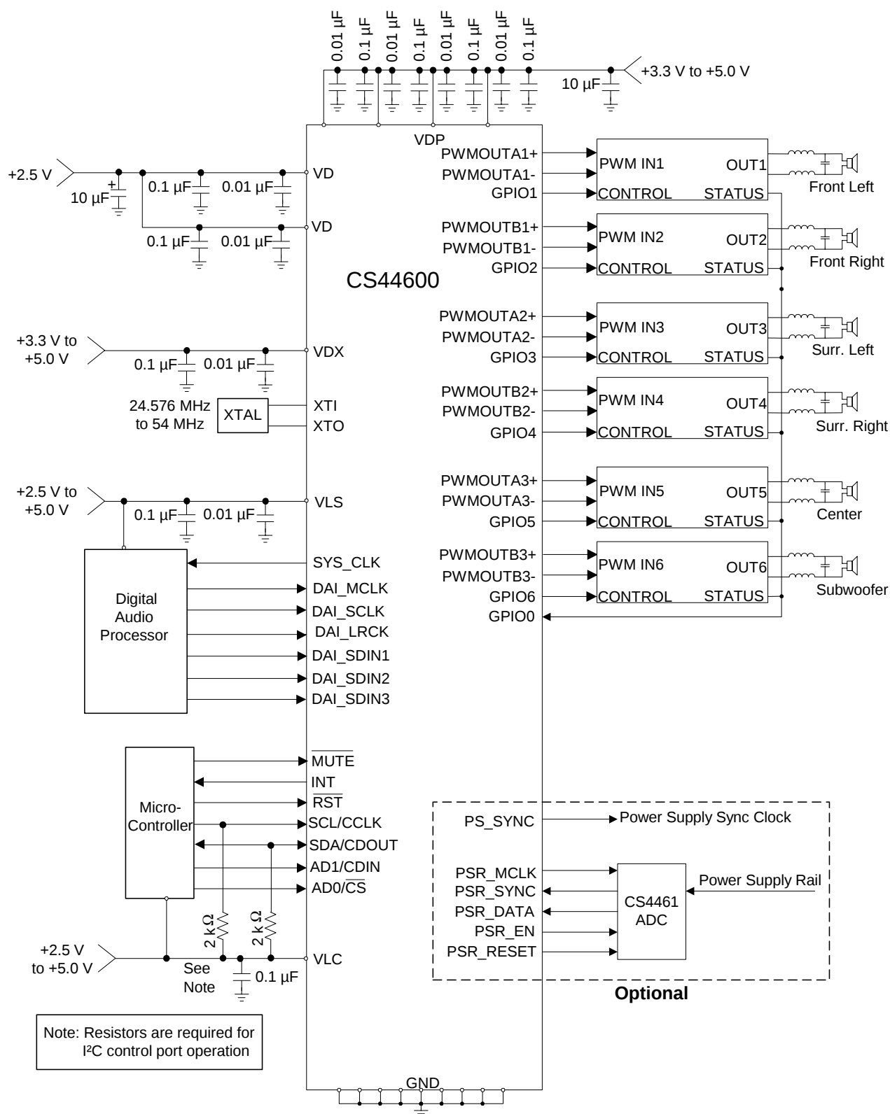
Figure 11. Typical Full-Bridge Connection Diagram
