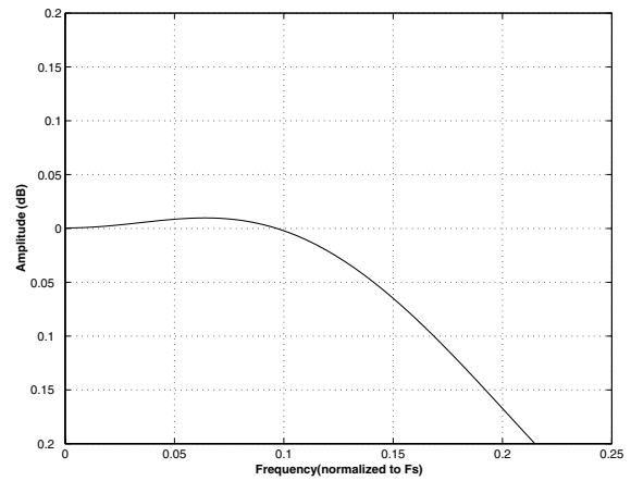
Figure 47. Quad-Speed (fast) Passband Ripple
