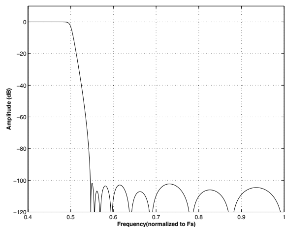
Figure 28. Single-Speed (fast) Stopband Rejection
