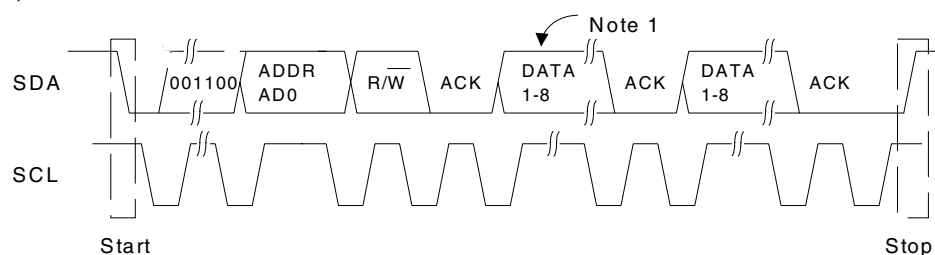
Figure 26. Control Port Timing, I 2 C Mode
