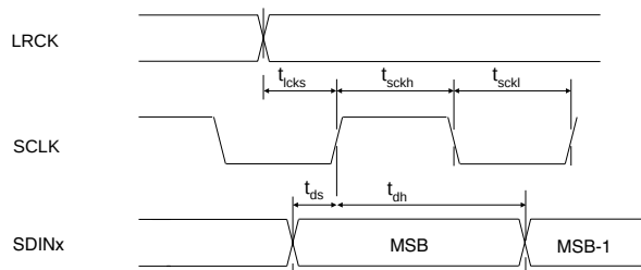
Figure 1. Serial Audio Interface Timing
