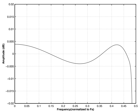
Figure 31. Single-Speed (fast) Passband Ripple
