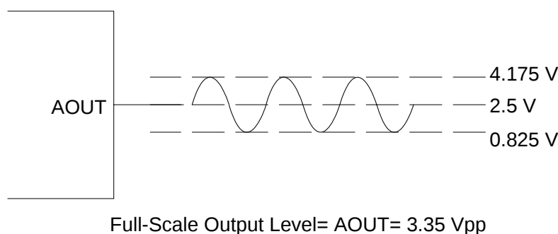
Figure 23. Full-Scale Output
