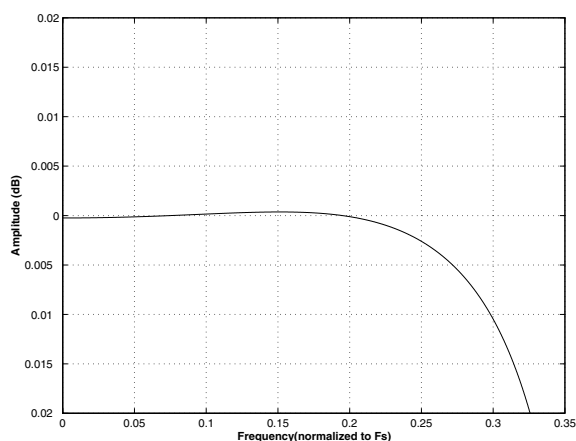
Figure 43. Double-Speed (slow) Passband Ripple
