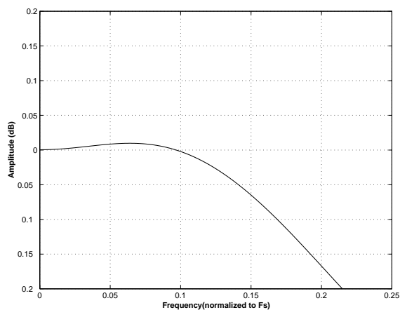
Figure 32. Quad-Speed (fast) Passband Ripple
