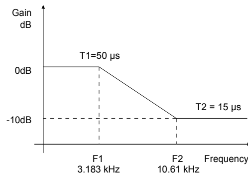
Figure 21. De-Emphasis Curve
