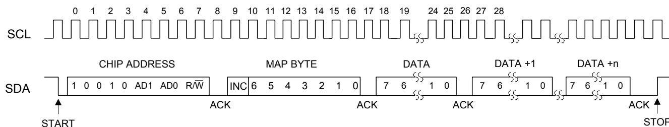
Figure 19. Control Port Timing, I²C Mode
