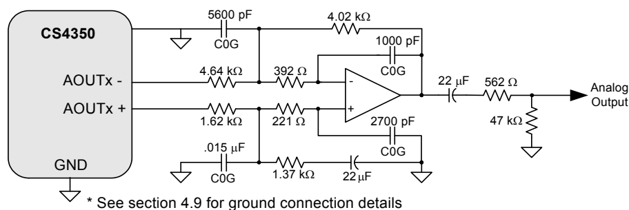
Figure 17. Differential to Single-Ended Output Filter
