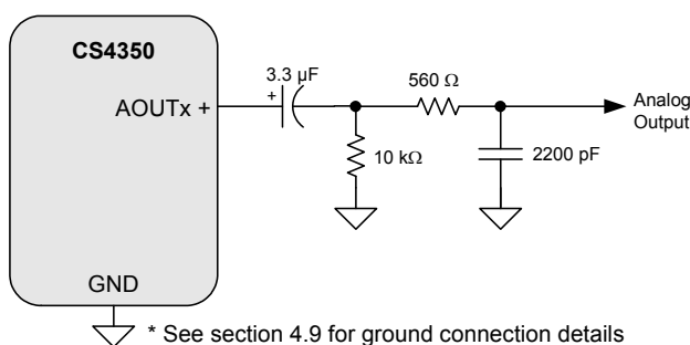
Figure 18. Passive Single-Ended Output Filter
