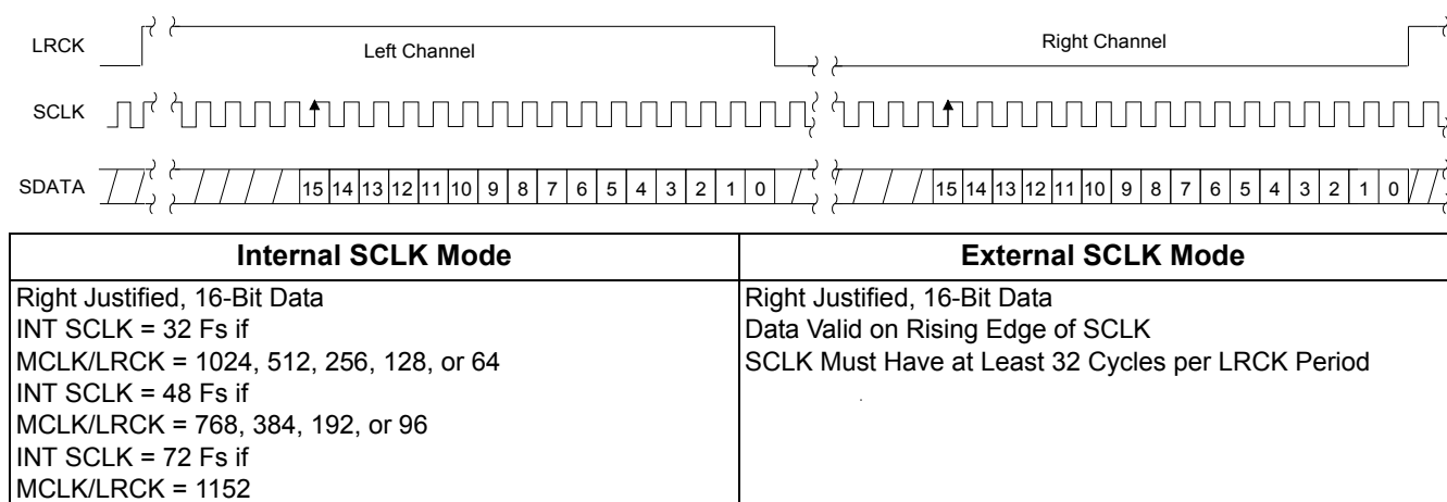
Figure 9. CS4348 Data Format (Right Justified 16)
