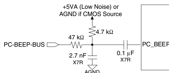
Figure 22. PC_BEEP Input
