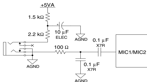
Figure 21. Microphone Input
