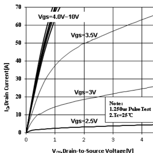
Figure 4. Typical output Characteristics
