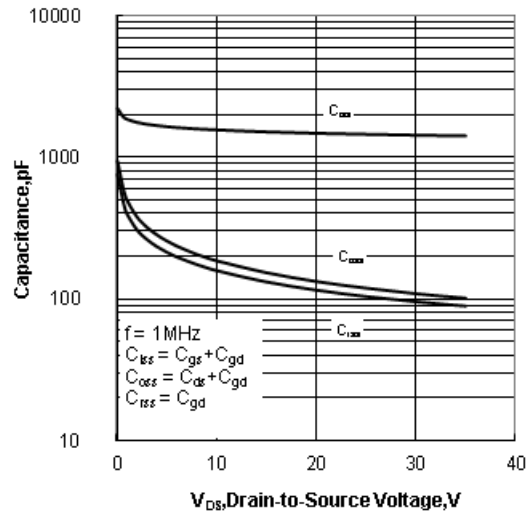
Figure 12. Capacitance Characteristics
