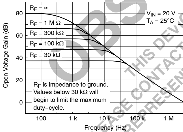
Figure 2. Error Amplifier Voltage Gain vs. Frequency Over RF
