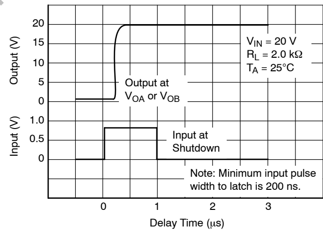
Figure 9. Turn-Off Delay from Shutdown
