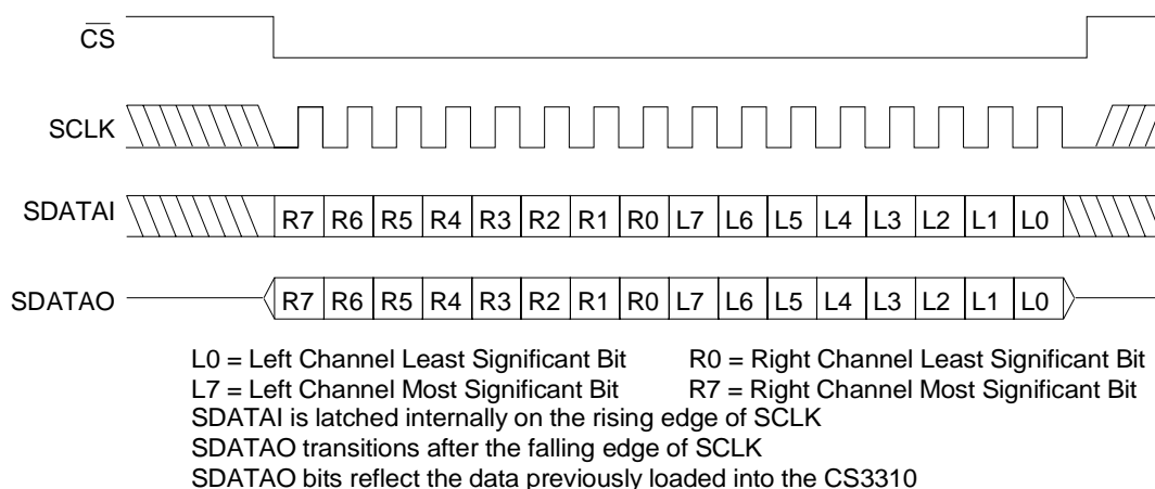
Figure 3. Serial Port Timing
