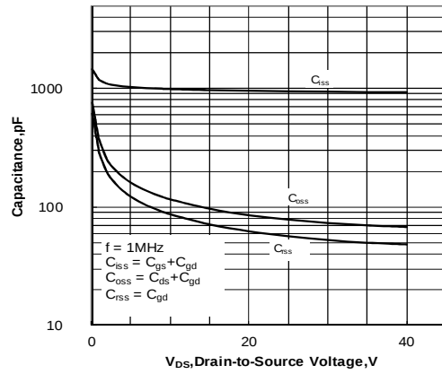
Figure 12. Capacitance Characteristics
