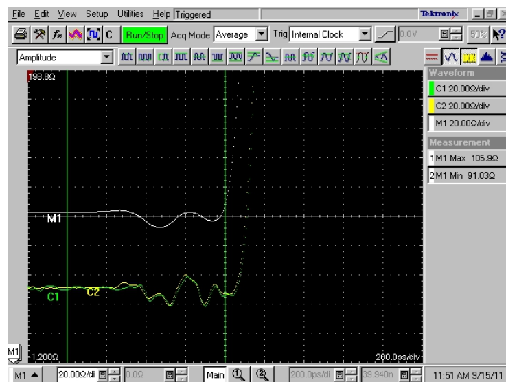
Figure 4 TDR Measurements for HDMI
