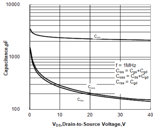
Figure 12. Capacitance Characteristics
