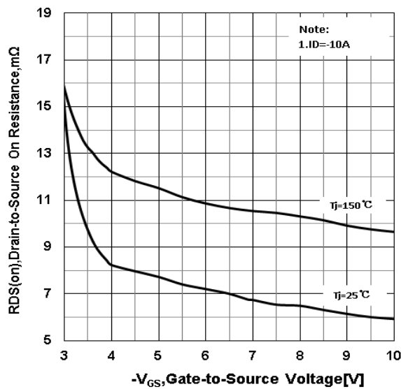
Figure 14 . Drain-to-Source On Resistance vs Gate Voltage
