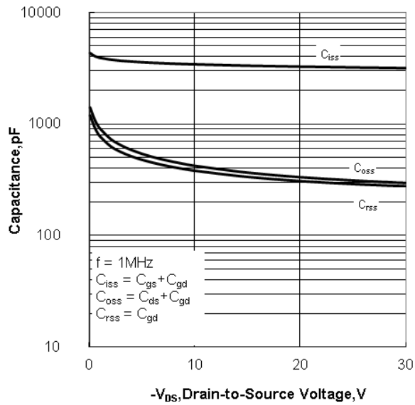
Figure 12. Capacitance Characteristics
