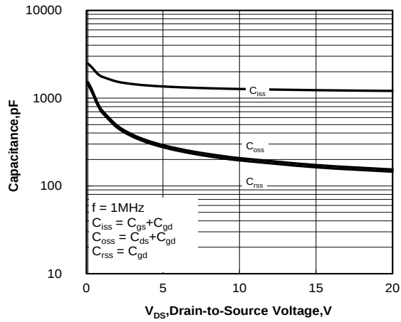
Figure 12. Capacitance Characteristics
