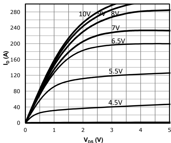
Fig 1: Output Characteristics
