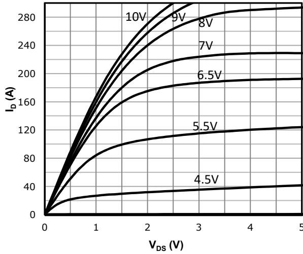
Fig 1: Output Characteristics
