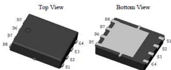
CRSM055N10L4
