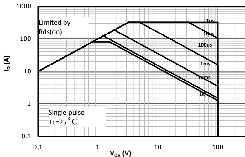
Fig 11: Safe Operating Area
