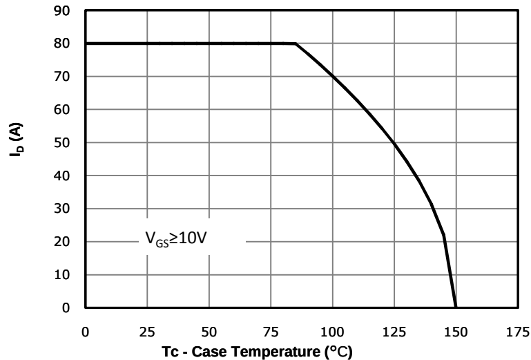
Fig 10: Drain Current Derating
