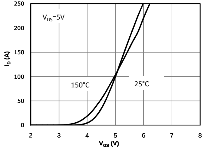
Fig 2: Transfer Characteristics
