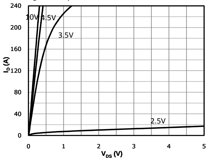
3.5V Fig 1: Output Characteristics
