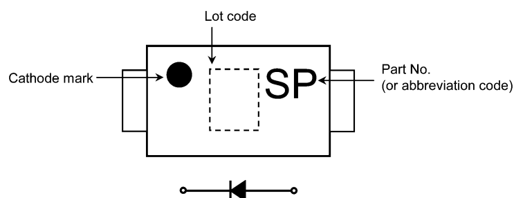
Fig. 7.1 Marking
