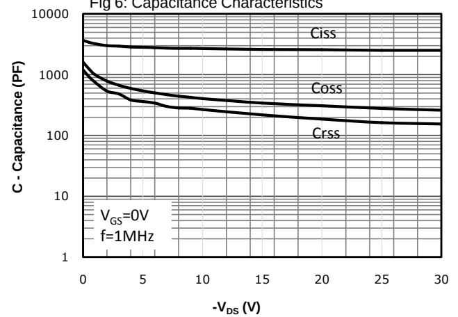
Fig 6: Capacitance Characteristics
