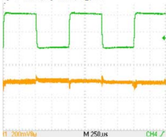
LOAD Transient
